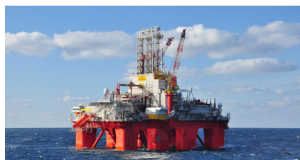
16 silencers in AISI 316 for Rolls Royce engine, Aker H6e rig
